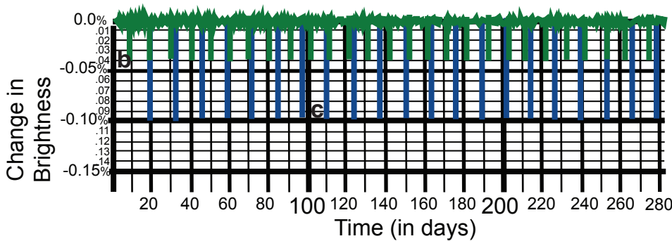
Kepler-11b and c
